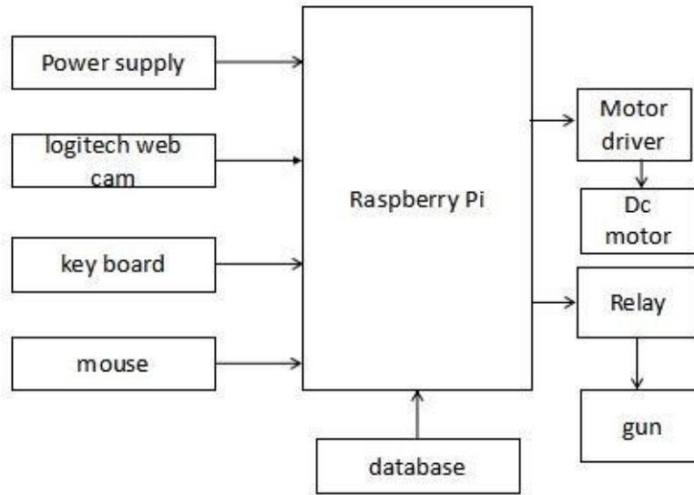
Fig. : Block diagram of the system.
