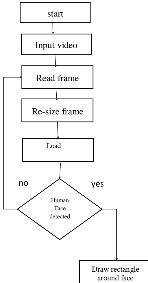
Fig: Flow diagram for face detection
