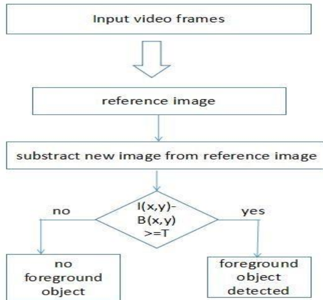
Fig: Flow diagram for background subtraction.
