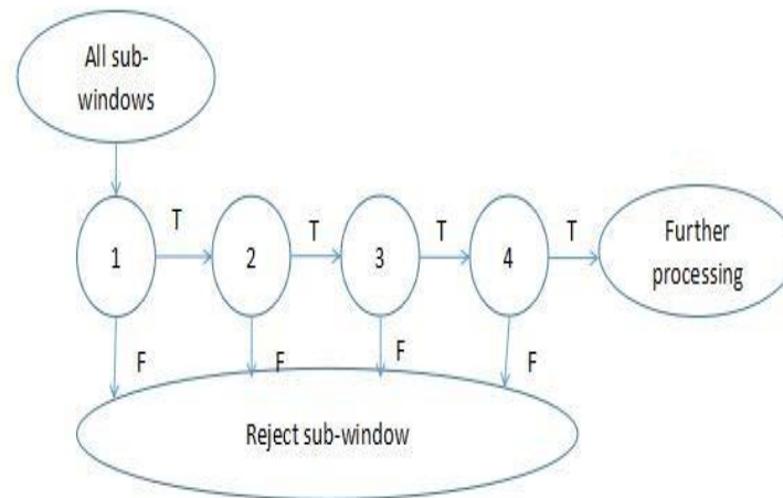
Fig: Stages of cascade classifier.
